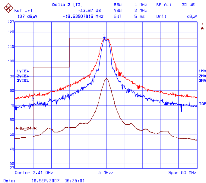
Plot 6.8.5.1(b) Band-Edge RF Radiated Emissions @ 3 m Low End of Frequency Band Rx Antenna Orientation: Horizontal
