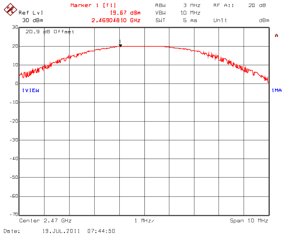
Plot 5.5.3.3. Peak Conducted Output Power Test Frequency: 2470 MHz
