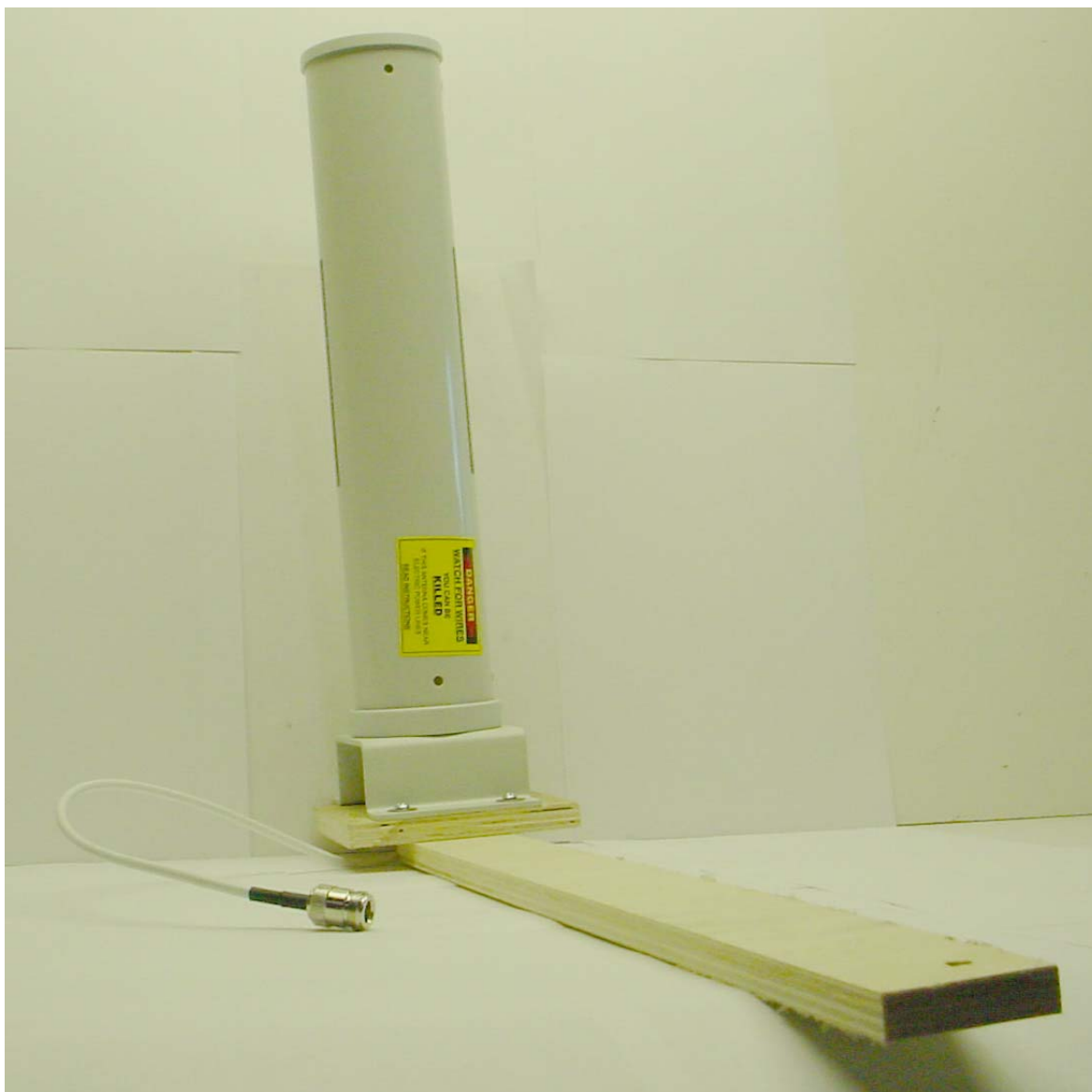
Maxrad Yagi Antenna (P/N: A24-Y18NF; Max. Antenna Gain = 15 dBi)
