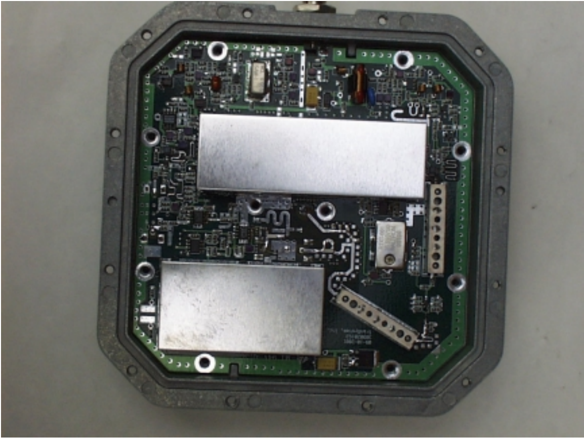
Board Top View
