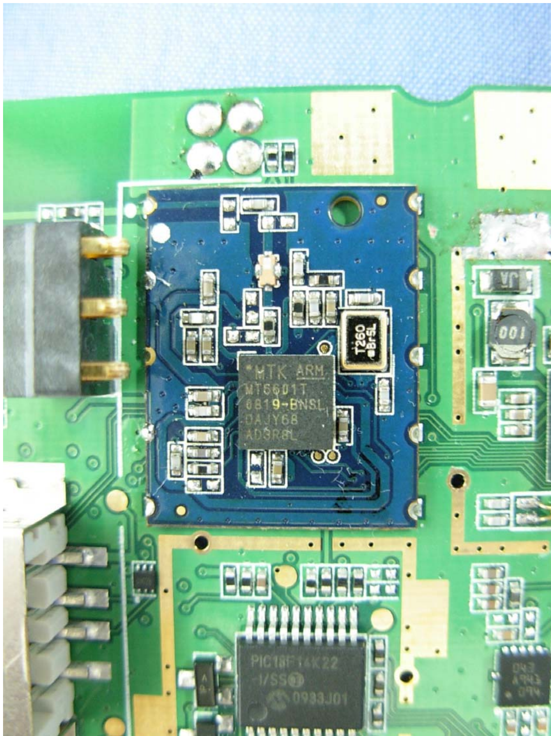
(11) EUT Photo
