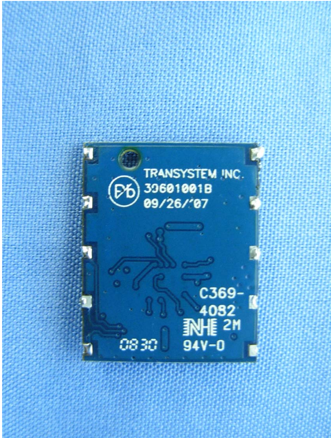
(22) EUT Photo
