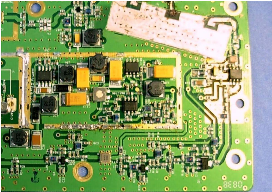
(11) EUT Photo
