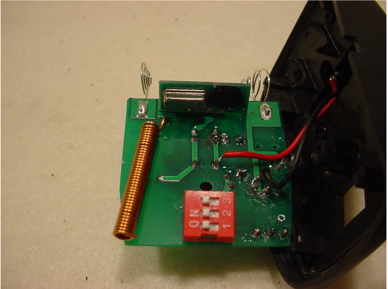
Figure 2: Internal – PCB Back
