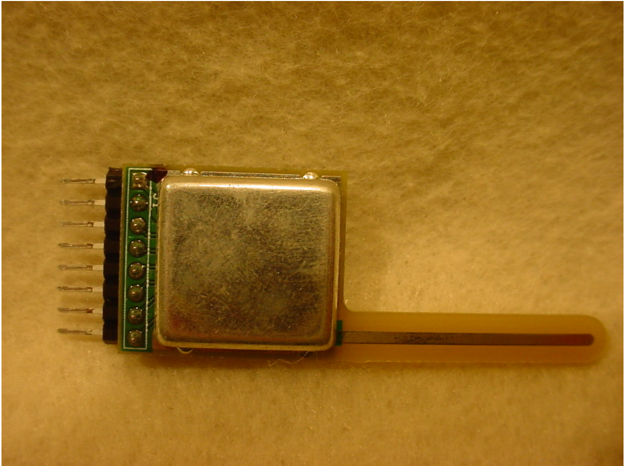
Figure 1: PCB Front
