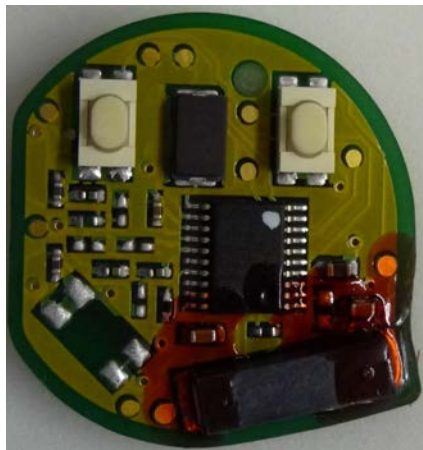
Figure 7.7 PCB assy (front view)
