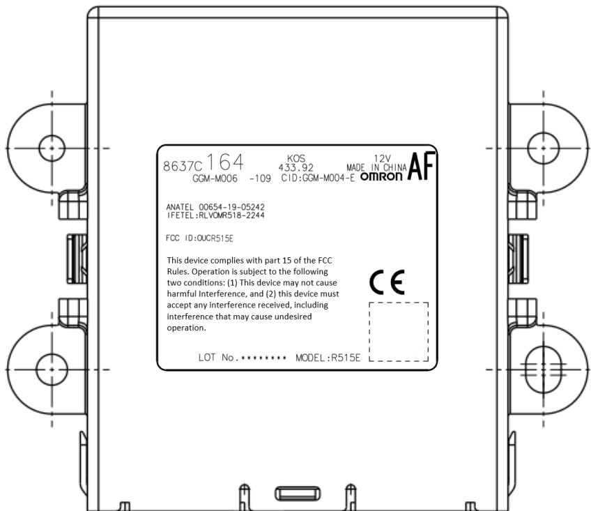
Figure 9.2 R515E appearance
