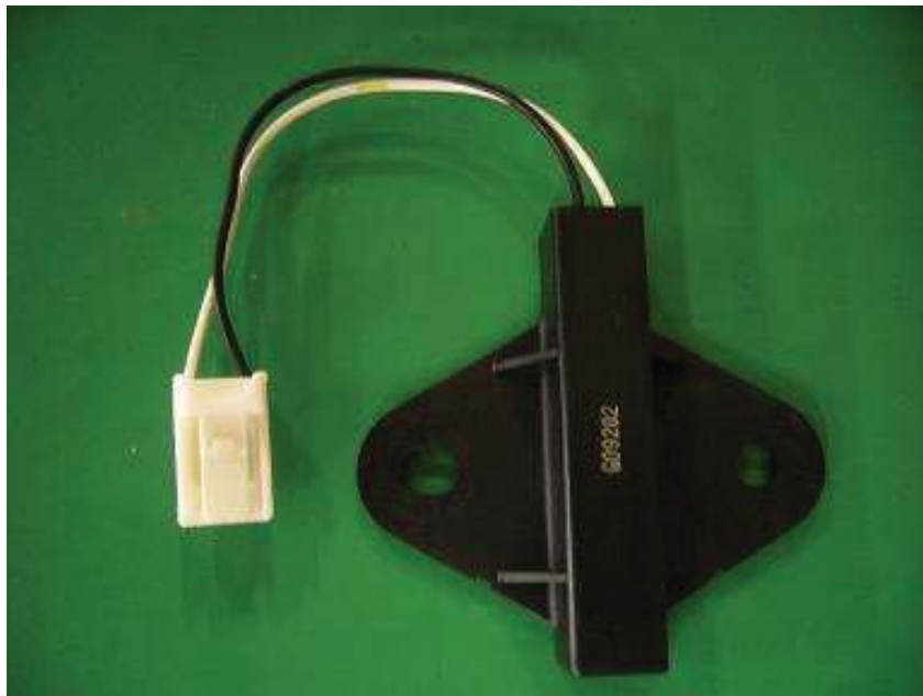
Figure 8.11 G8D-841M-ANT(InF,InR,T/G) appearance (front view)
