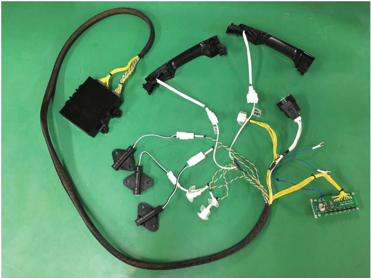
Figure 8.15 Connection picture
