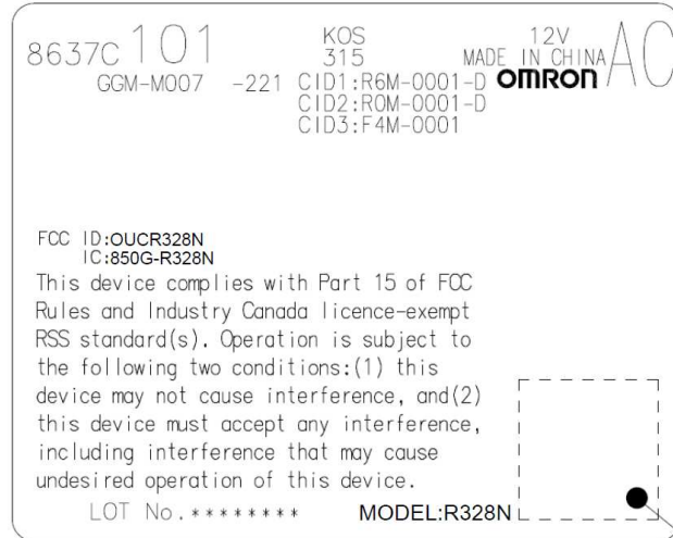
Figure 9.1 R328N Label
