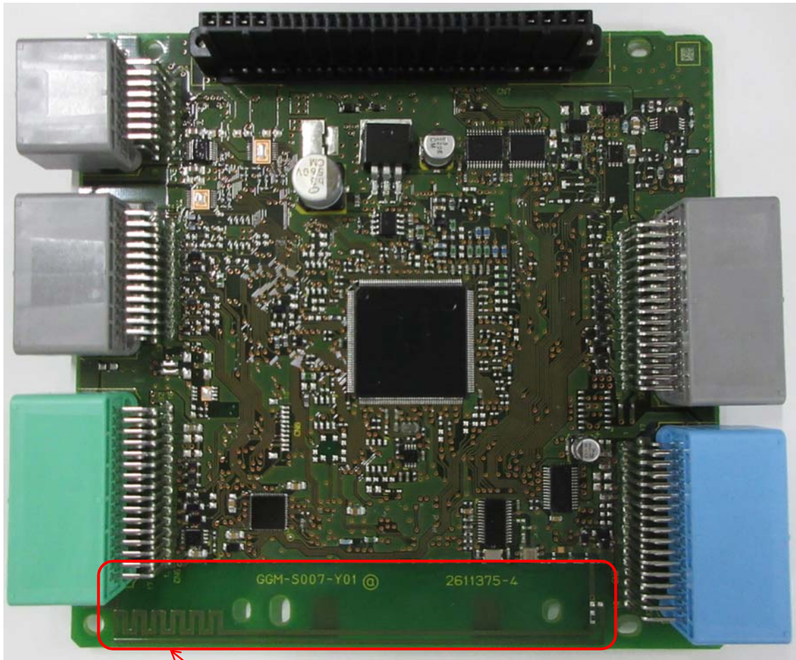
Pattern Antenna
