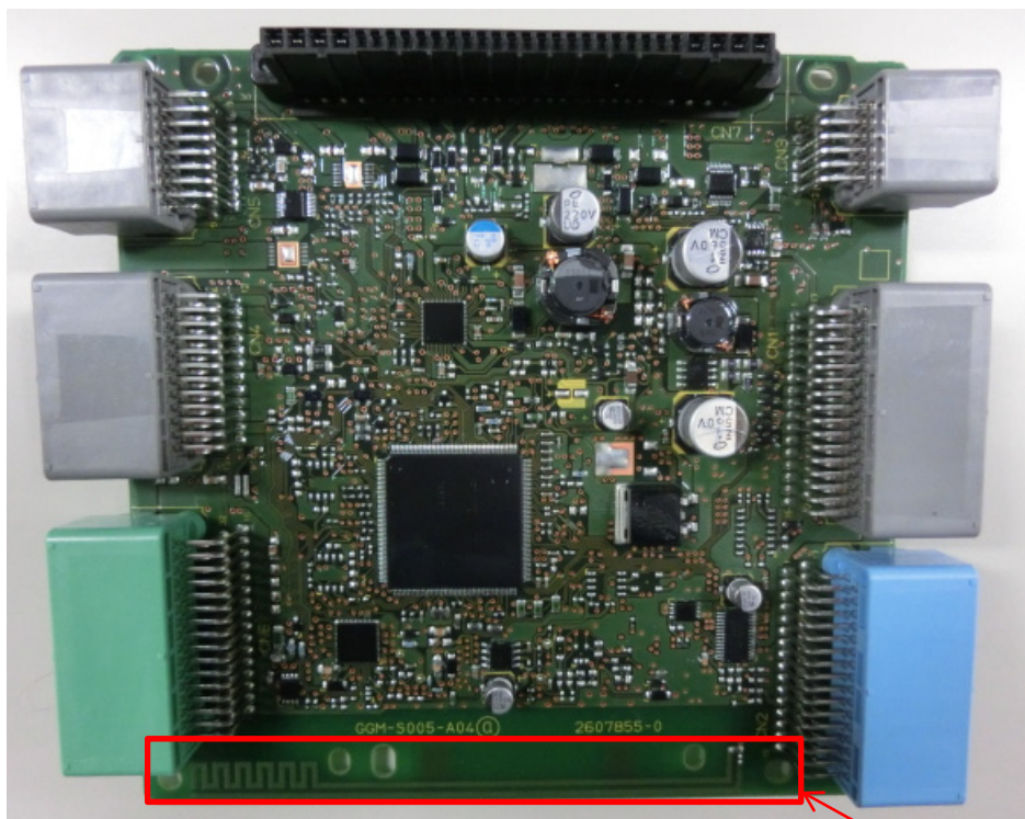
Figure 8.1 K56R0 PCB assy (top view)
