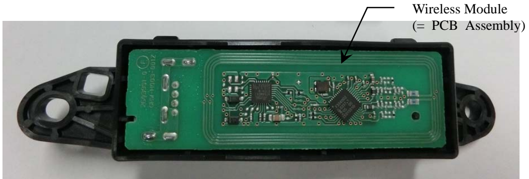
Figure 8.6 Wireless module location
