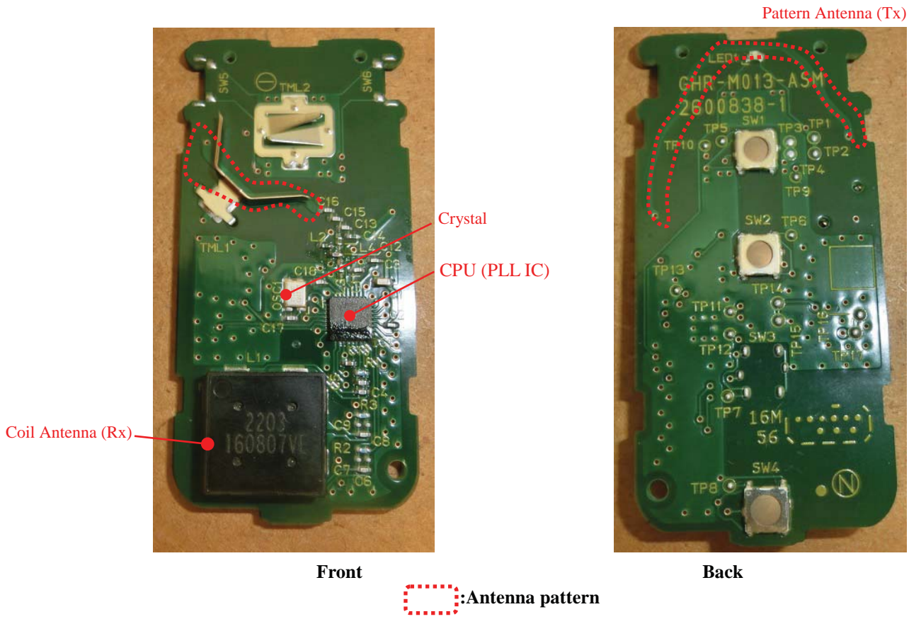
Figure 8.2 FOB appearance (PCB)
