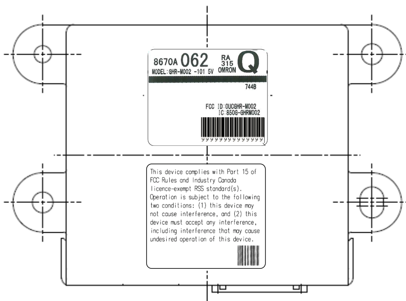
Figure 9.2 GHR-M002 label location
