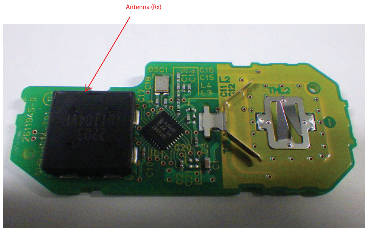
Figure 8.2 GHR-H015-T PCB assy (bottom view)
