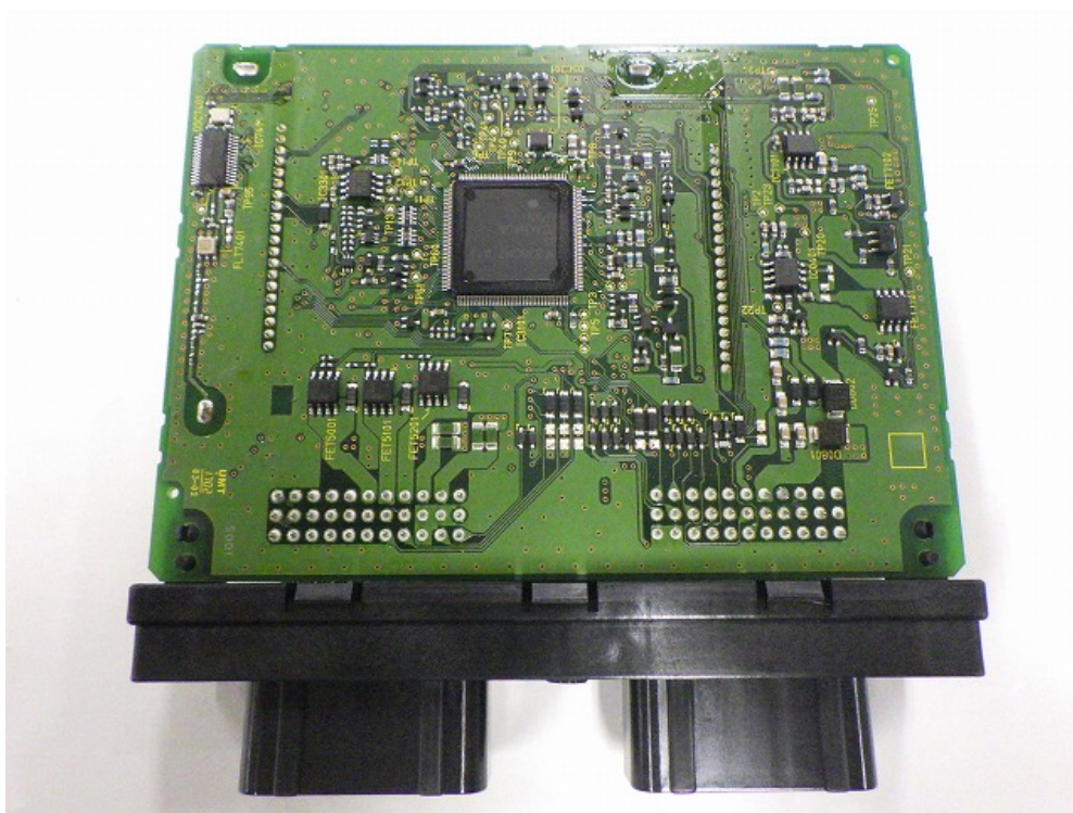
Figure 8.2 GHR-H015-R PCB assy (bottom view)
