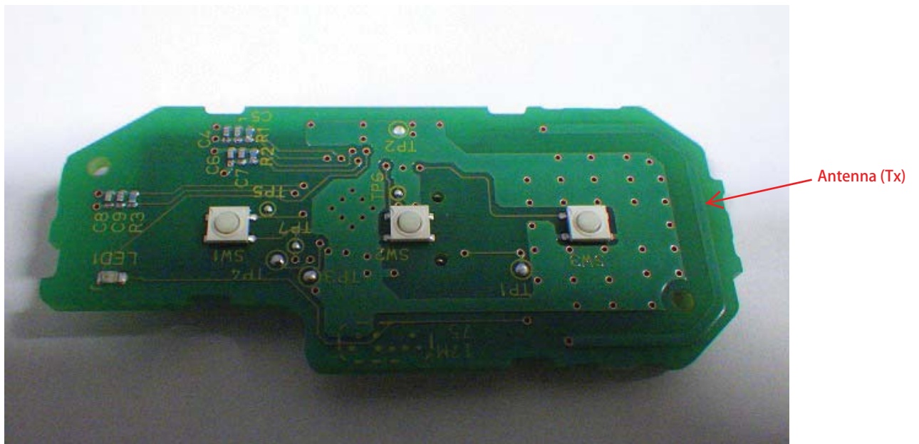
Figure 8.1 GHR-H014-T PCB assy (top view)
