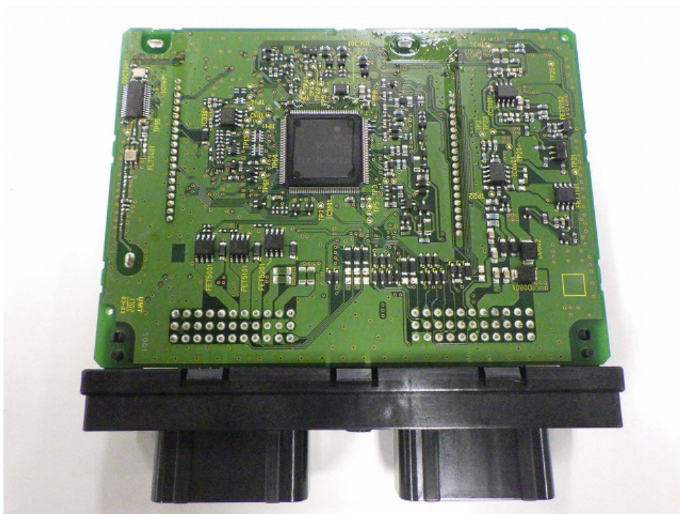
Figure 8.2 GHR-H014-R PCB assy (bottom view)
