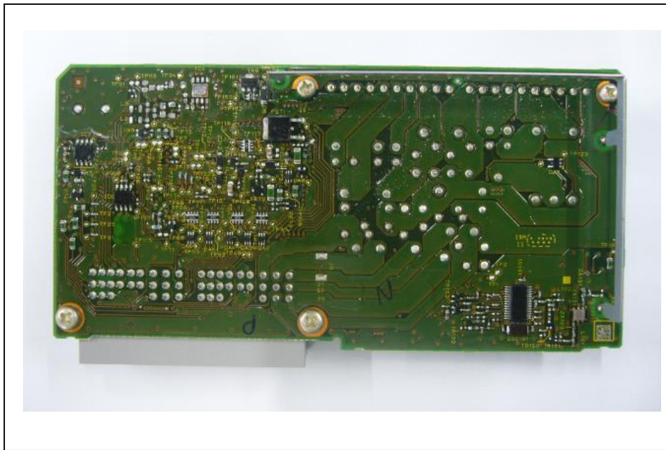
Figure 7.4 PCB ASSY (back view)
