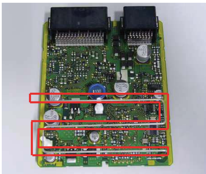
Figure 8.3.2 GGM-M007 integral antenna ( for UHF receiving ) location
