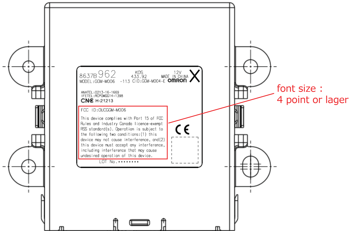
Figure 9.2 GGM-M006 appearance
