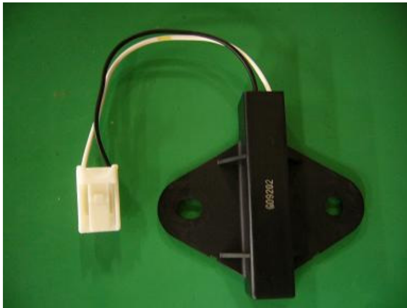
Figure 8.7 G8D-841M-ANT appearance (front view)
