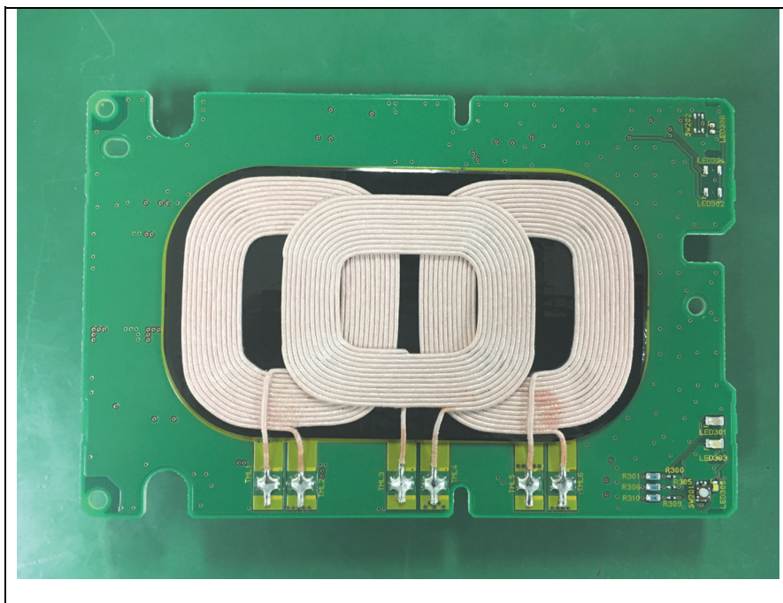
Figure 8.7 Wireless Charger Module [6] (bottom view)
