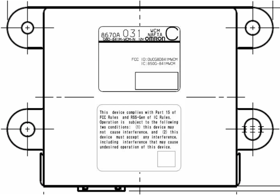
Figure 9.2 G8D-841M-WCM-N appearance
