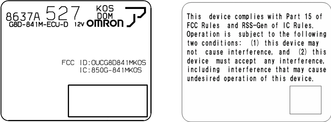
Figure 9.1 Labels
