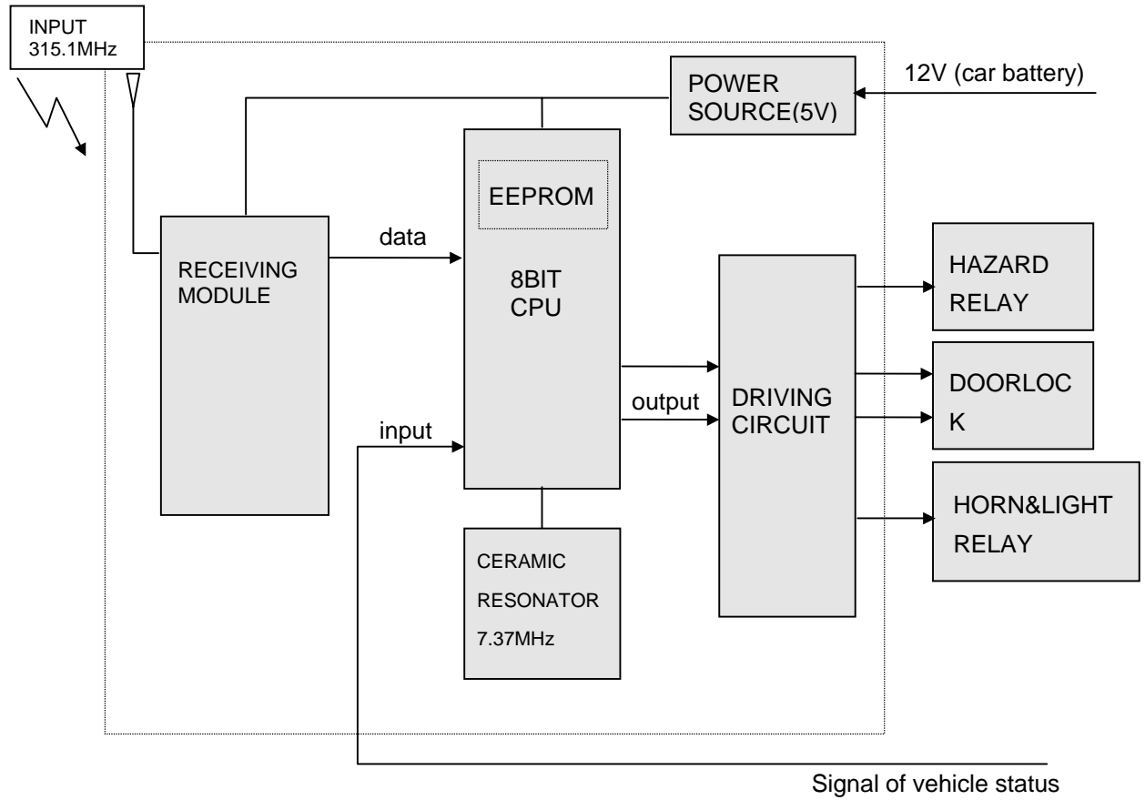
Figure 3.1 block diagram of the receiver
