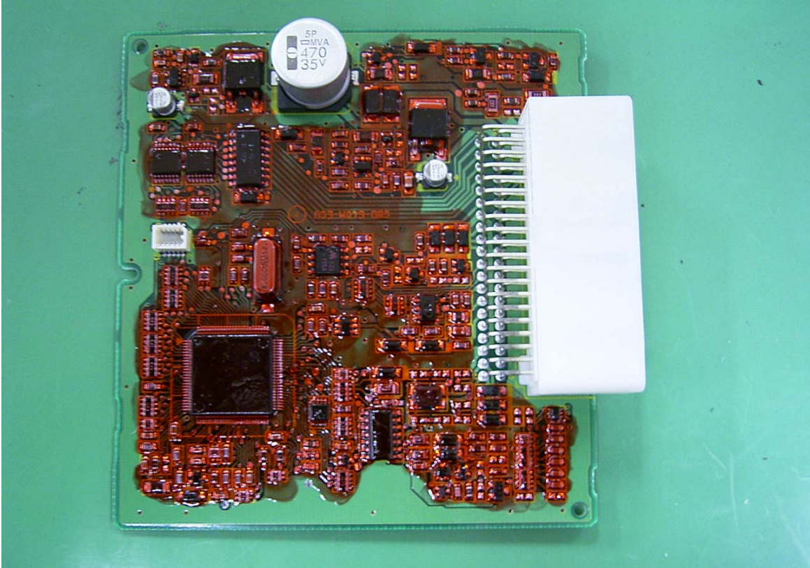
Figure 8.3 G8D-640M-ECU PCB assy (front view)
