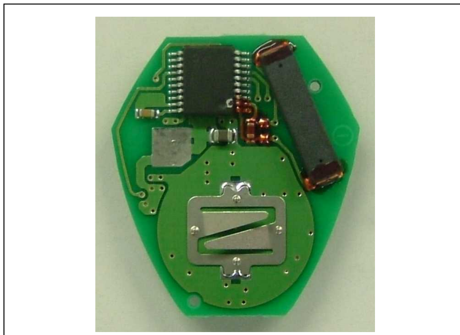
Figure 7.7 PCB assy (back view)
