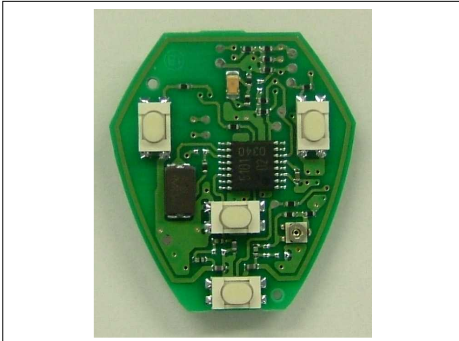
Figure 7.6 PCB assy (front view)
