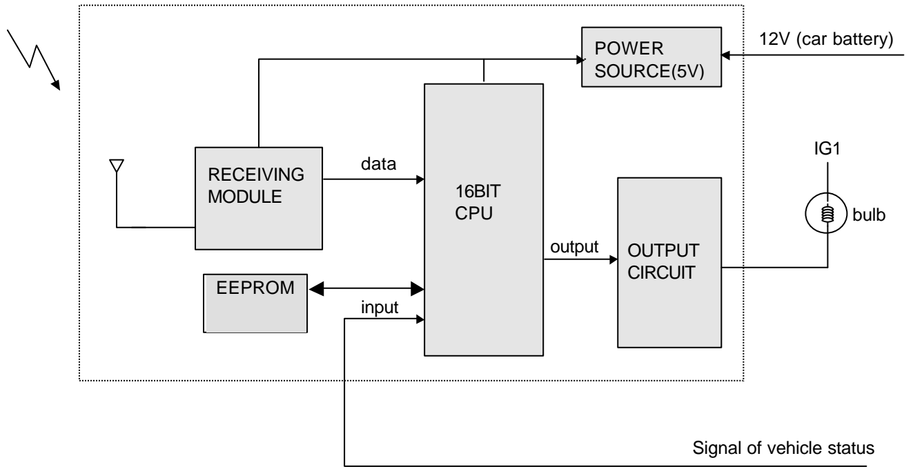
Figure 3.1 block diagram of the receiver
