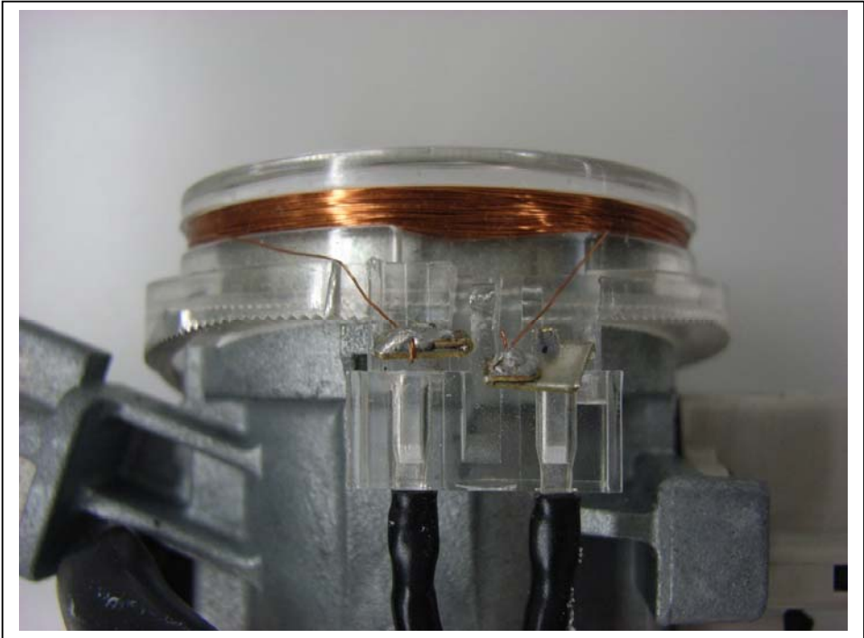
Coil Antenna
