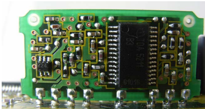
Figure 9.2.3 RF Part (UHF receive ) PCB(front view)
