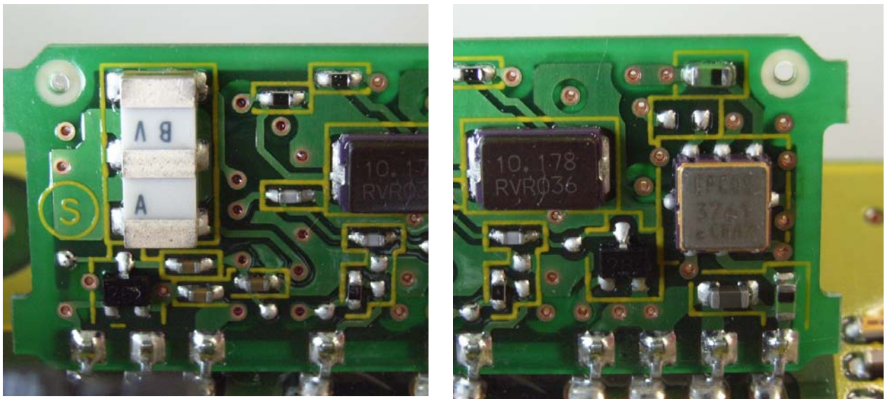
Figure 9.2.5 RF Part (UHF receive ) PCB(back view) close up
