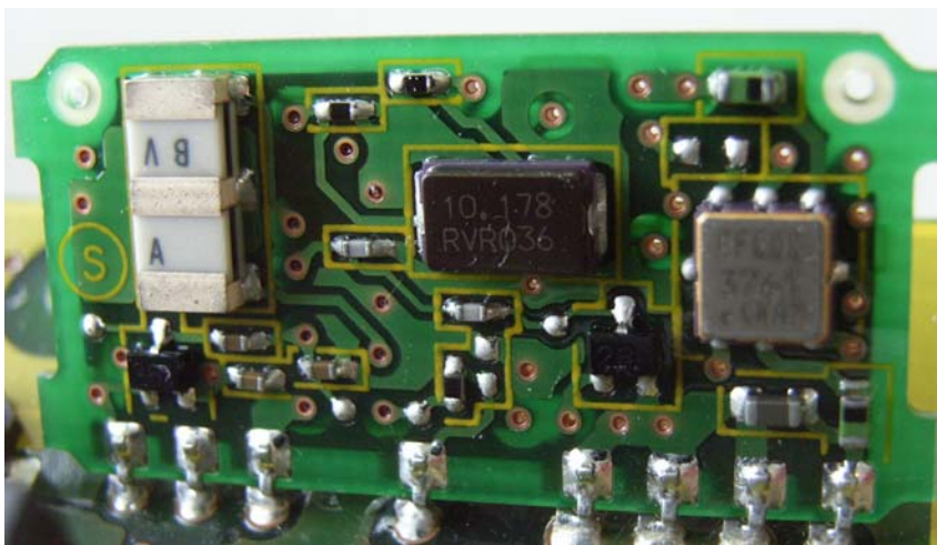
Figure 9.2.4 RF Part (UHF receive ) PCB(back view)
