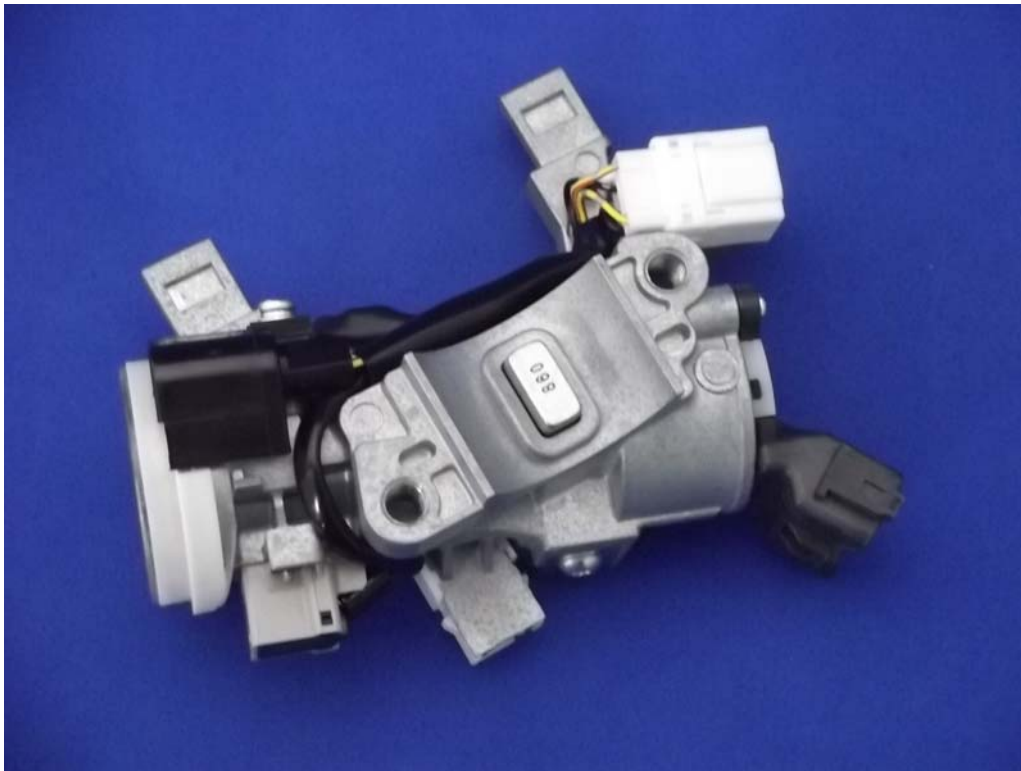
Side View2
