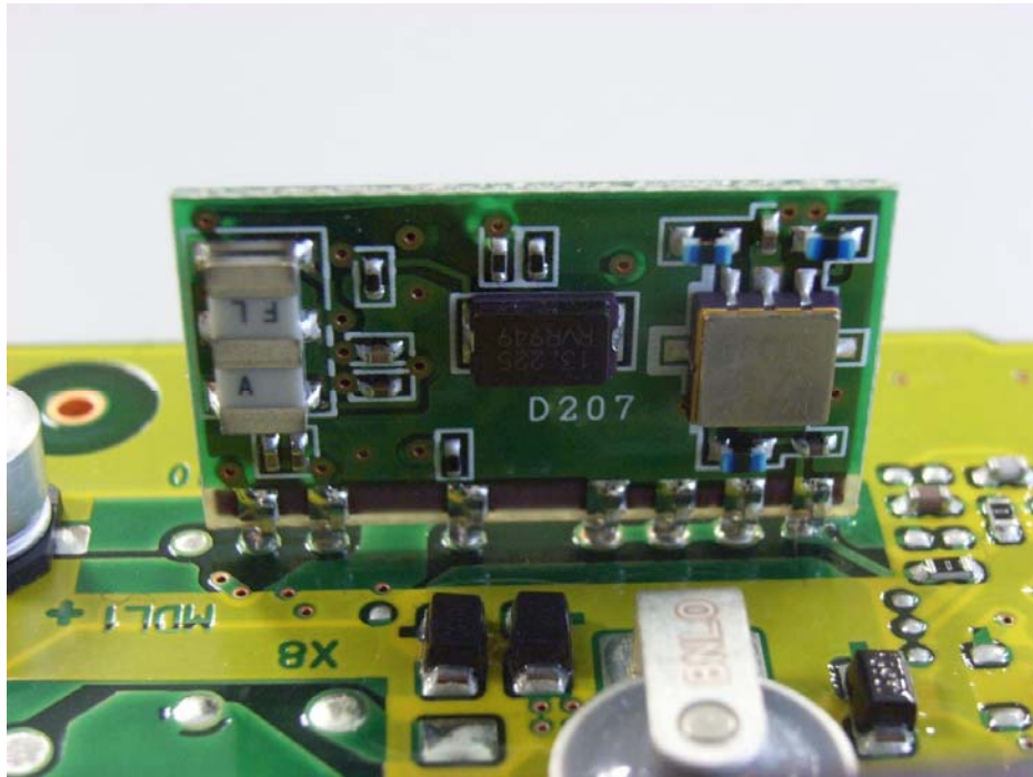
UHF Receiving Circuit(Front)
