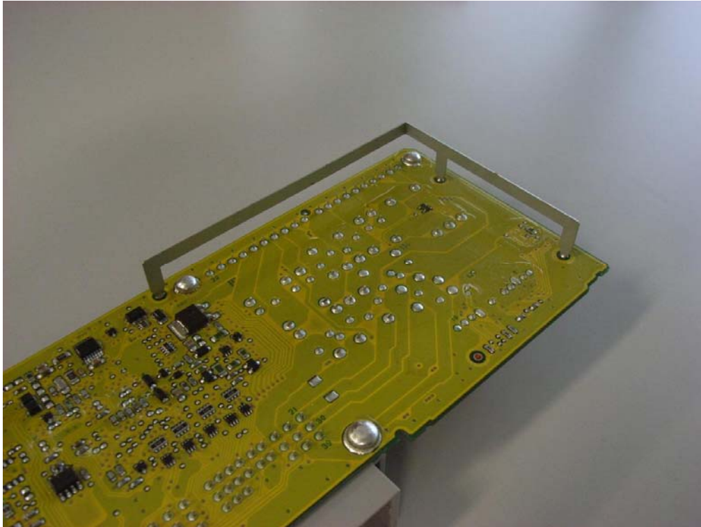
UHF Receiving-antenna
