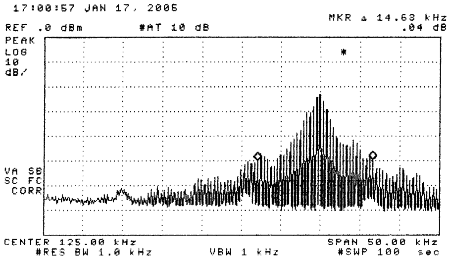
Figure 6.3. Measured bandwidth of the DUT. (repeated pulses)
