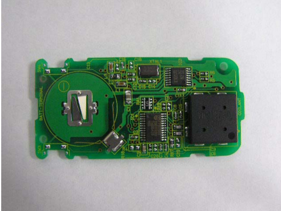
G8D-644M-KEY-N PCB assy (front view)
