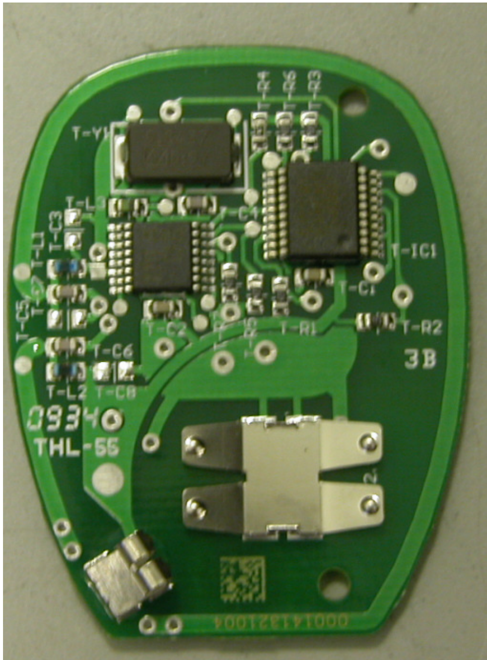
Figure 3. Top side of PCB
