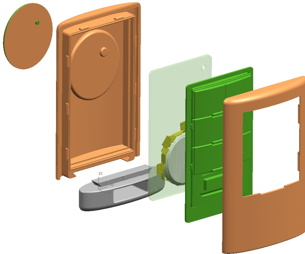
Figure 7. Mechanical Explosion of Transmitter
