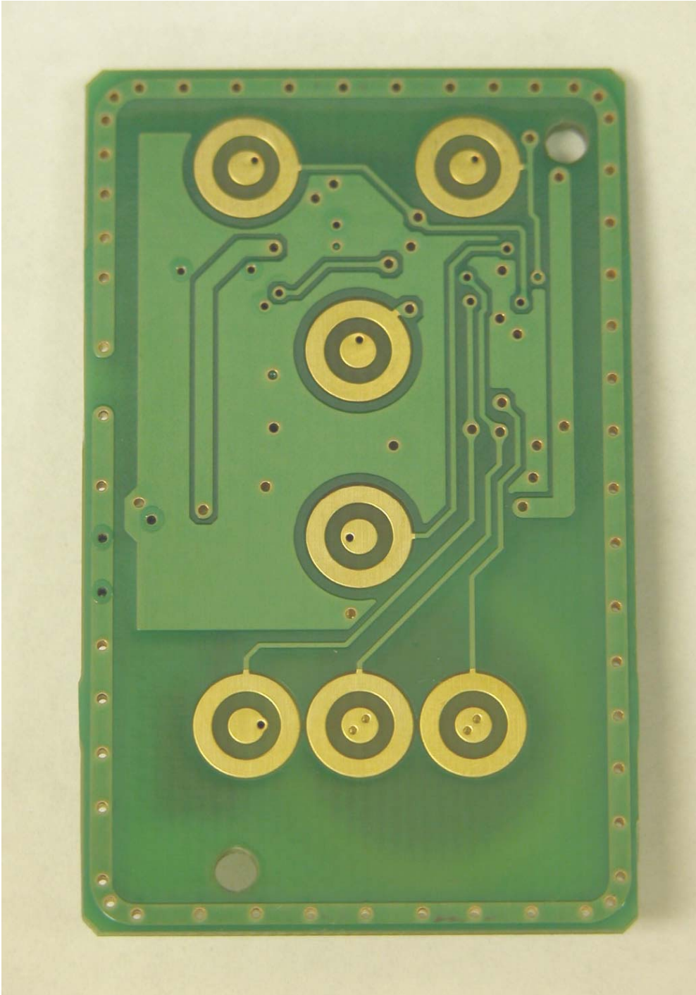
Figure 6. Bottom side of PCB
