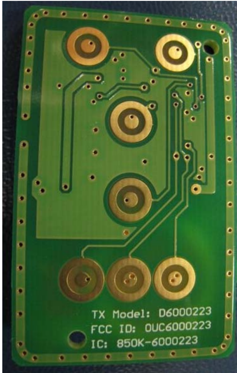
Figure 6. Bottom side of PCB
