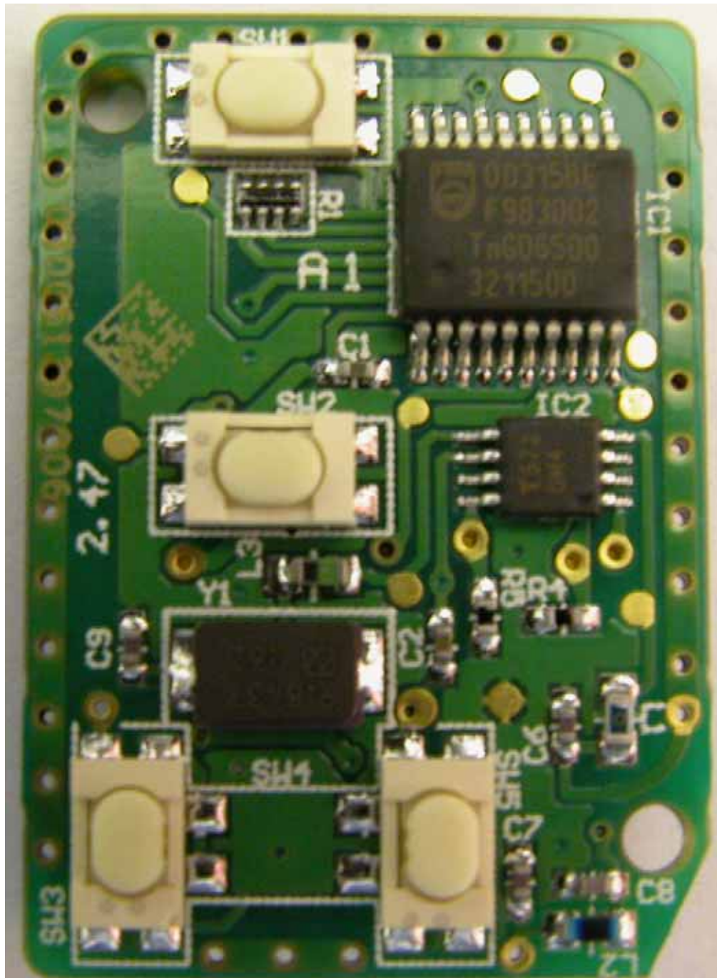
Figure 5. Topside of five-button PCB
