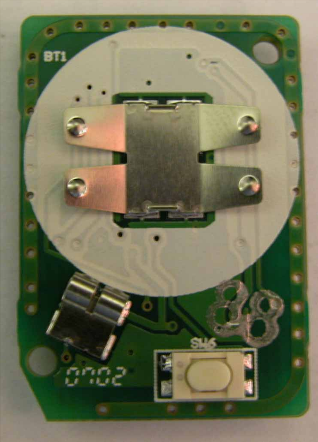
Figure 6. Bottom side of PCB
