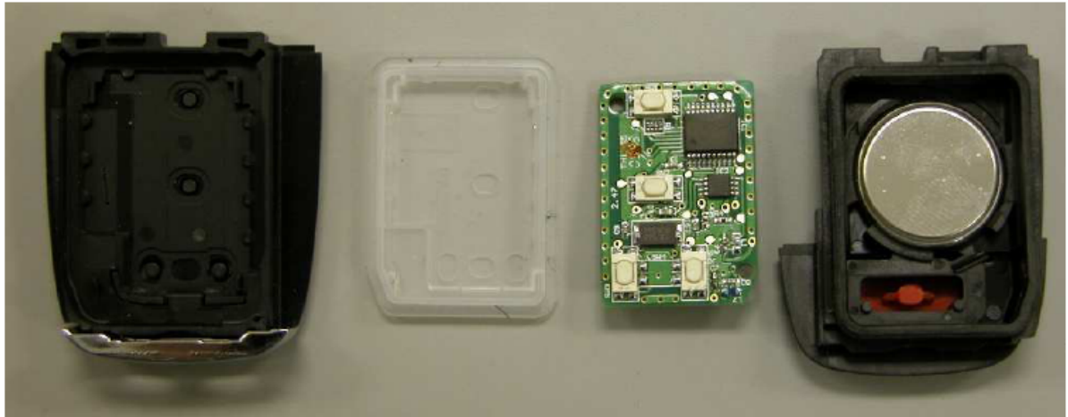
Figure 8 Individual pieces of final assembly
