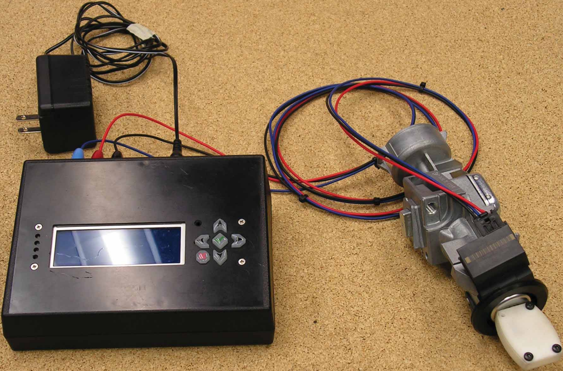
DUT with Harness + test box, employing Antenna DS5T-15607-BA and Metal Lock Cylinder
