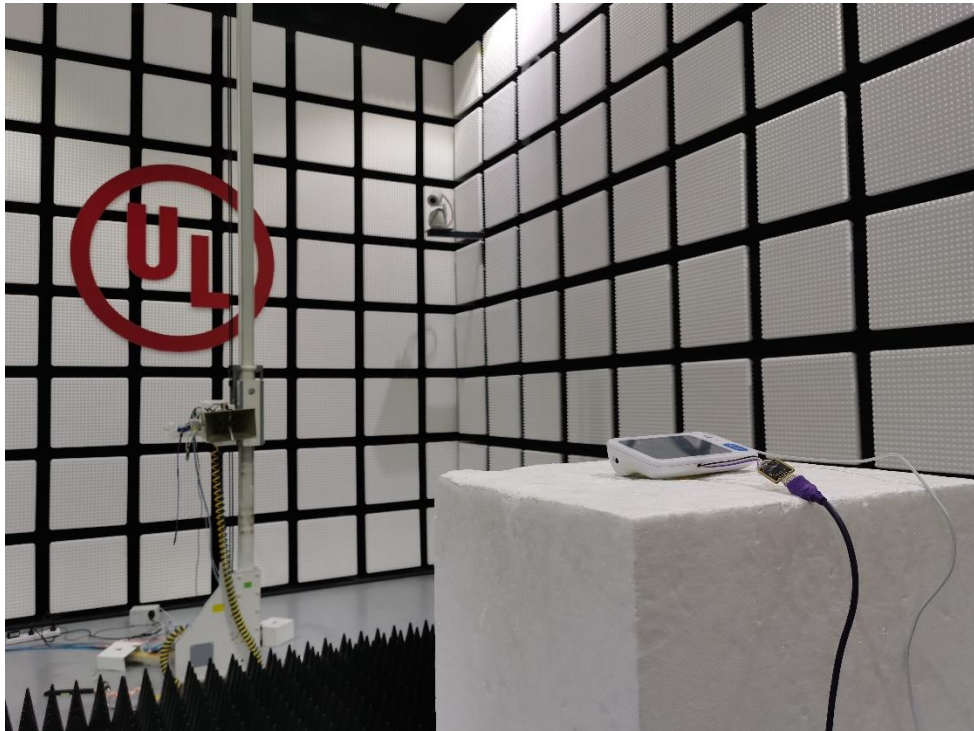
Radiated Disturbance Setup (Above 1 GHz – X axis)
