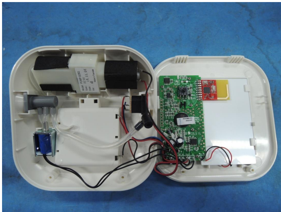
Internal Photo of TMB-1491-BT
