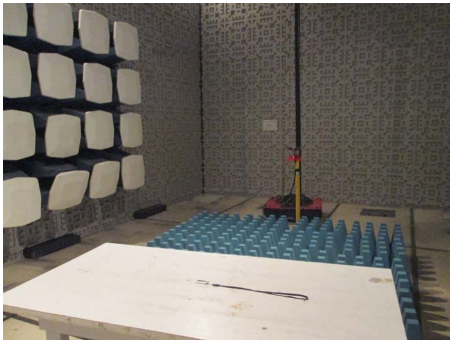
TEST SETUP OF RADIATED EMISSION-3
