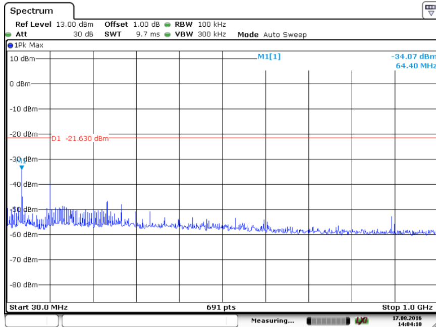
30MHz – 1GHz
