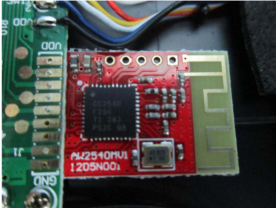
View of Product-7(Bluetooth Module)
