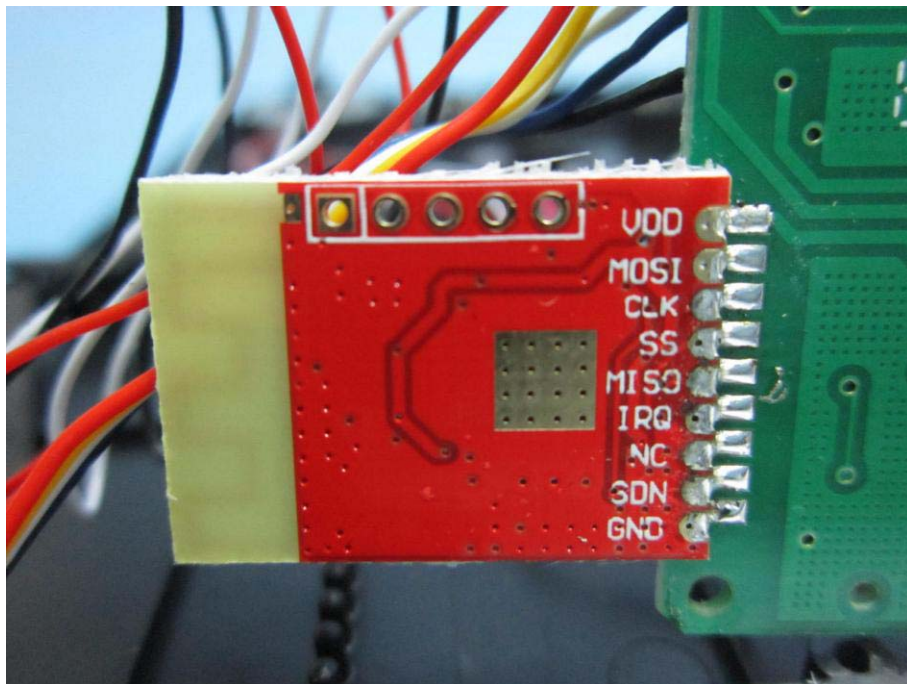
View of Product-8(Bluetooth Module)
