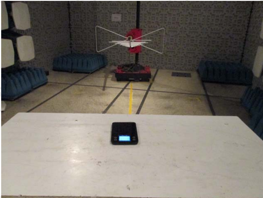
TEST SETUP OF RADIATED EMISSION-2
